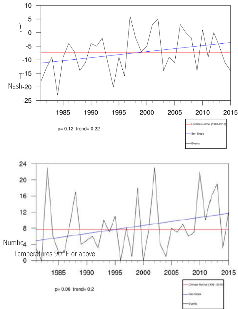
Figure 4: In a study conducted using data in Nashua, climatological trends suggest the minimum temperature and the number of days 90F or above are both increasing. Source: Presentation by Kelly Neugent, 2016. Source: Neugent, 2016.
